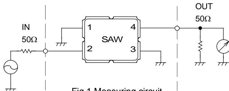
Fig.1 Measuring circuit
